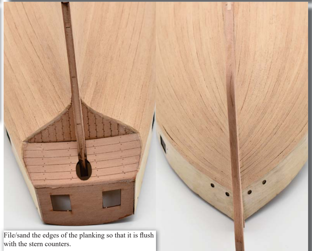
Second planking complete and sanded smooth using medium to fine grit abrasive paper. The planks were also filled with filler and sanded smooth.
