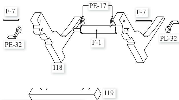
Main mast aft bitts assembly
